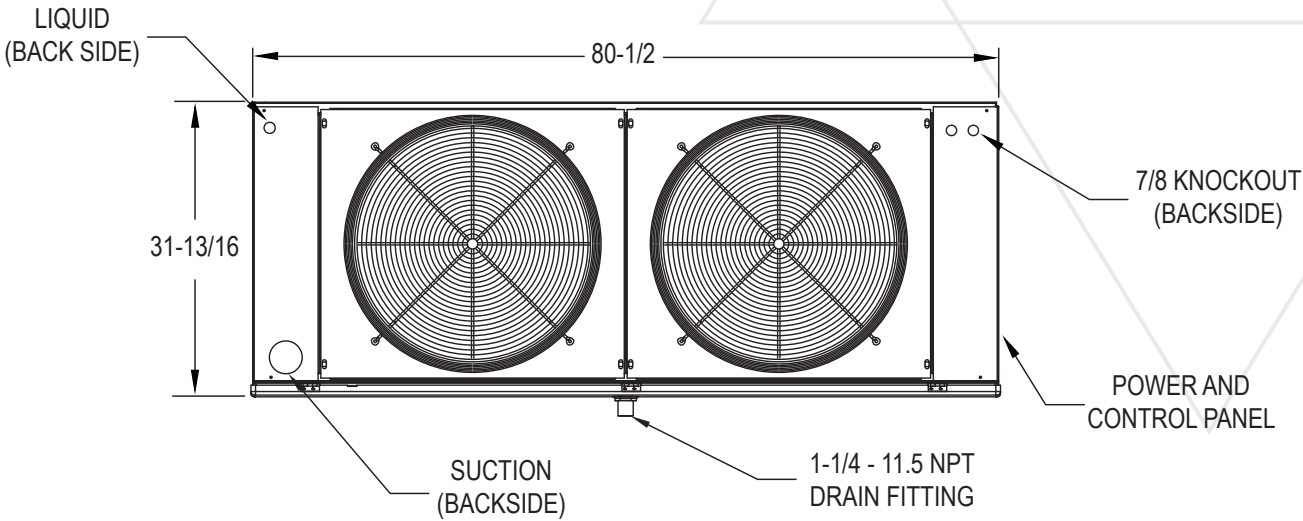
Figure 2: Two Fan
