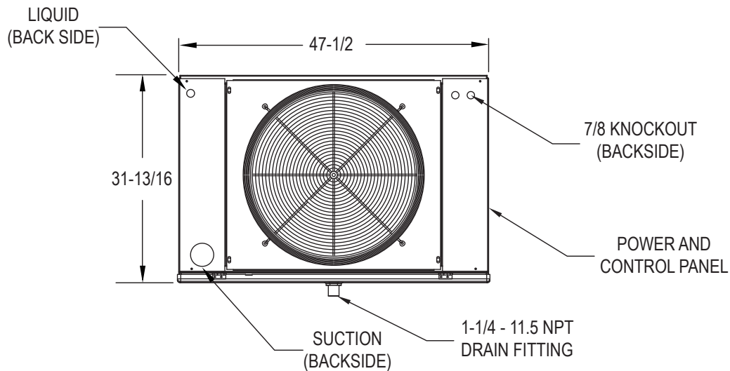
Figure 1: Single Fan
