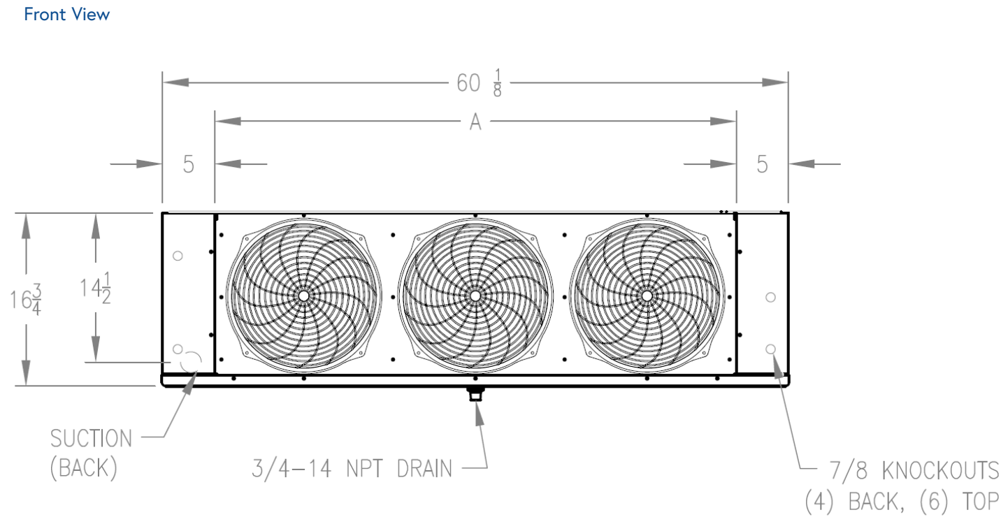
Figure 3 - Three Fan
