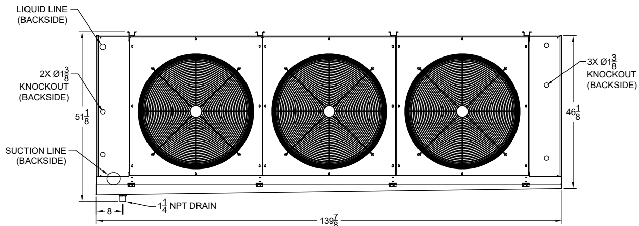
Figure 3: Three Fan
