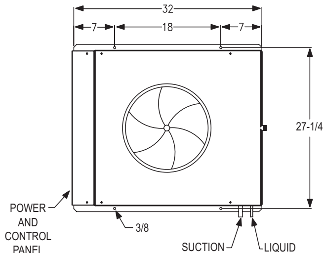
Figure 1 - Single Fan
