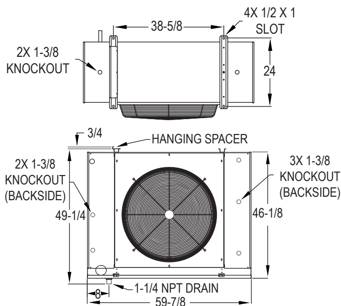
FIGURE 1 - SINGLE FAN
