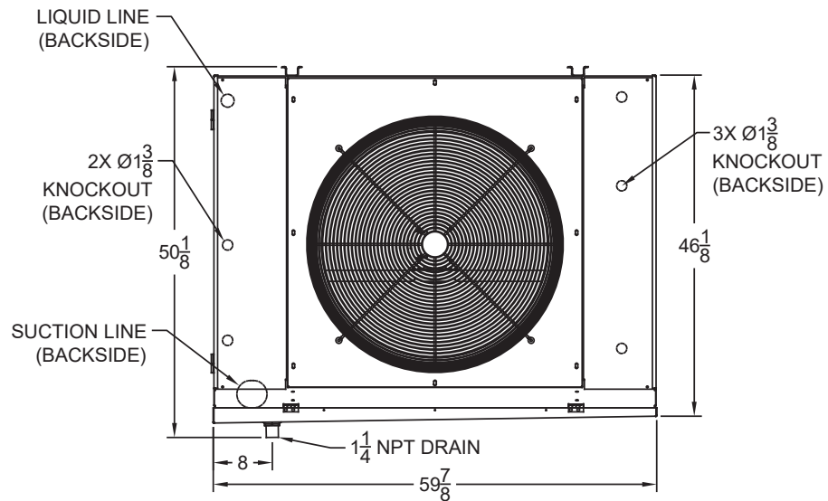
Figure 1: Single Fan
