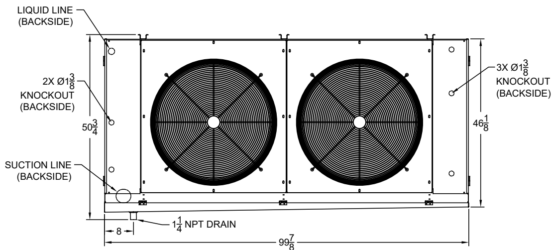
Figure 2: Two Fan
