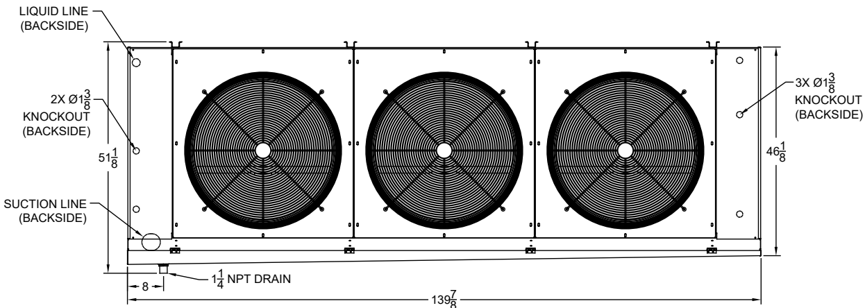
Figure 3: Three Fan
