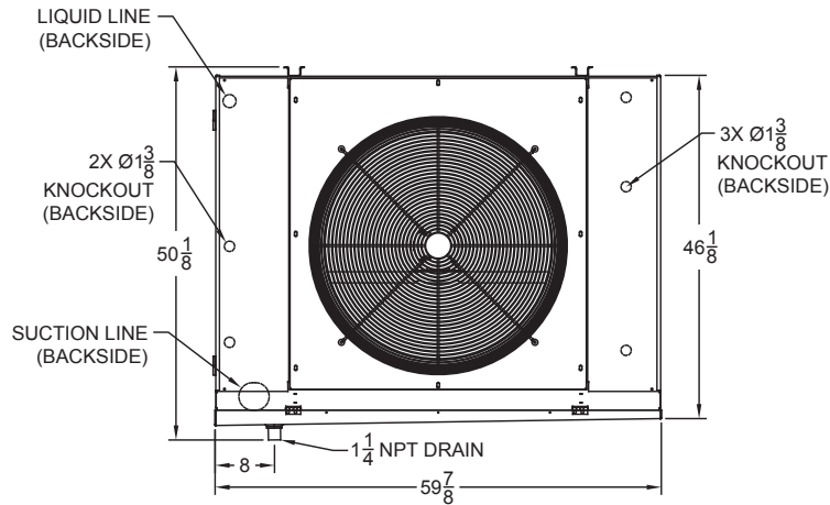
Figure 1 - Single Fan
