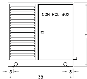
FRONT VIEW - 1 FAN MODEL DC/DL/DS
