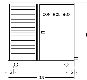
FRONT VIEW - 1 FAN MODEL DC/DL/DS
