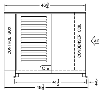
RIGHT SIDE VIEW MODEL DC/DL/DS
