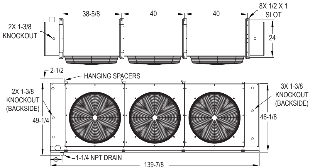
Figure 3 - Three Fan
