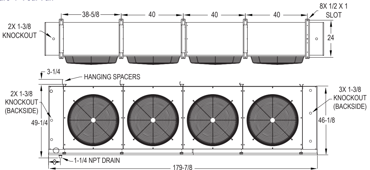
Figure 4- Four Fan
