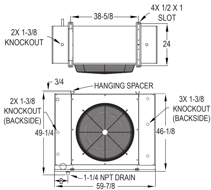
Figure 1 - Single Fan
